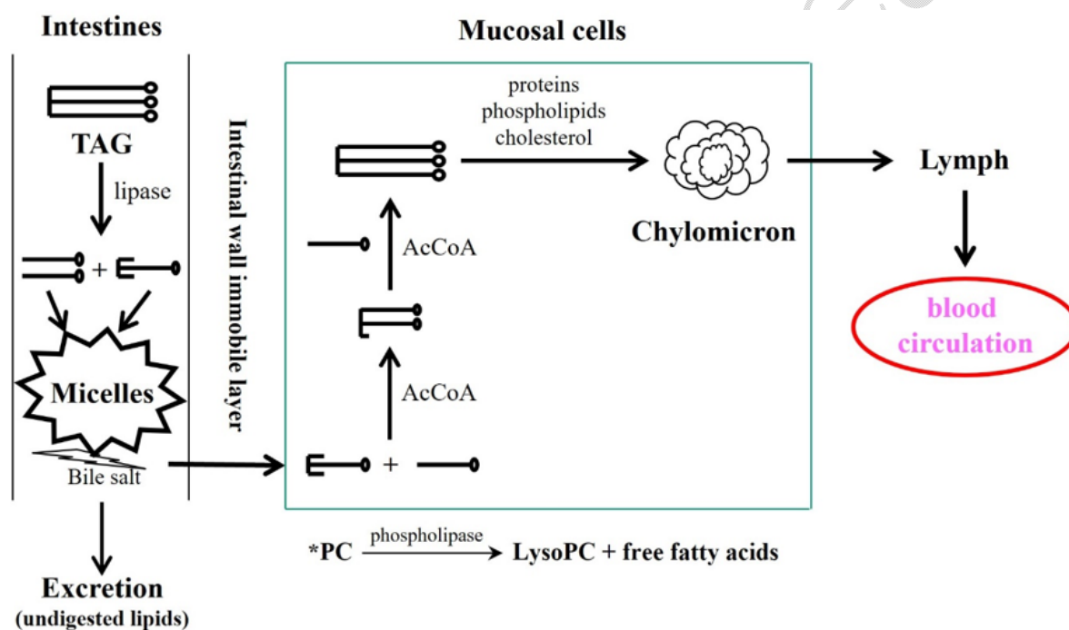
Figure 1. The various elements in the digestion and absorption of dietary lipids (in supplements or food). 33, 34
