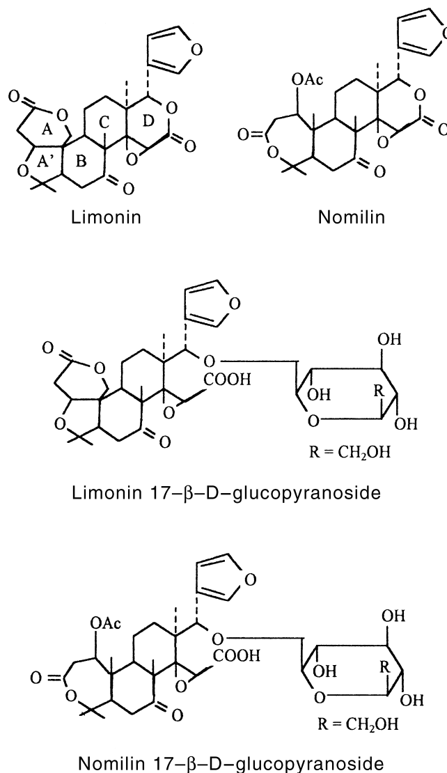
Figure 1. Chemical structures of limonin, nomilin and their glucoside derivatives.
