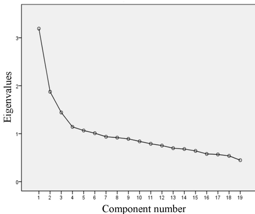
Supplementary figure 1. A scree plot of eigenvalues versus component number.
