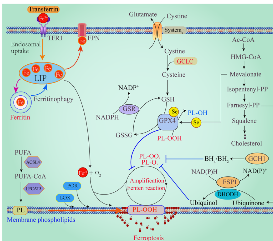
Figure 1. Molecular mechanism of ferroptosis. The transferrin receptor (TFR) facilitates the entry of \text{Fe}^{3+} into the cell, which is reduced to \text{Fe}^{2+} by metalloredutase (STEAP3) in the endosome and transported into the labile iron pool (LIP). Excess iron from LIP is stored in ferritin which can be degraded by ferritinophagy. In addition, ferroportin (FPN) facilitates \text{Fe}^{2+} export. Free PUFA are activated by acyl-coenzyme A (CoA) synthetase long chain family member 4 (ACSL4) and lysophosphatidylcholine acyltransferase 3 (LPCAT3) to generate membrane phospholipids (PL). PL undergoes lipid peroxidation and forms phospholipid hydroperoxides (PLOOH) via non-enzymatic (Fenton reaction) and enzymatic (lipoxygenases (LOX) and/or cytochrome P450 oxidoreductase (POR)) processes. PLOOH can react with cellular labile \text{Fe}^{2+} to generate alkoxyl and peroxy radicals, which can react with other PUFA and results in the propagation of PLOOH production. The classical ferroptosis-inhibiting axis includes uptake of cystine via the system xc- cystine-glutamate antiporter, which is crucial for glutathione (GSH) synthesis. Glutathione peroxidase 4 (GPX4) converts PLOOH to PL-OH by the use of reduced GSH as a substrate and protects cells from oxidative stress. Oxidized glutathione (GSSG) is reduced to GSH via glutathione-disulfide reductase (GSR) using electrons provided by NADPH. Other ferroptosis suppressive mechanisms include farnesyl-diphosphate farnesyltransferase 1 (GCH1)/ di/tetrahydrobiopterin (BH 2 /BH 4 ) pathway, the ferroptosis suppressor protein 1 (FSP1)-ubiquinone system and mevalonate pathway, which mediate inhibition of lipid peroxidation and protect cells from ferroptosis induction. Ac-CoA, Acetyl-CoA; HMG-CoA, 3-hydroxy-3-methylglutaryl CoA
