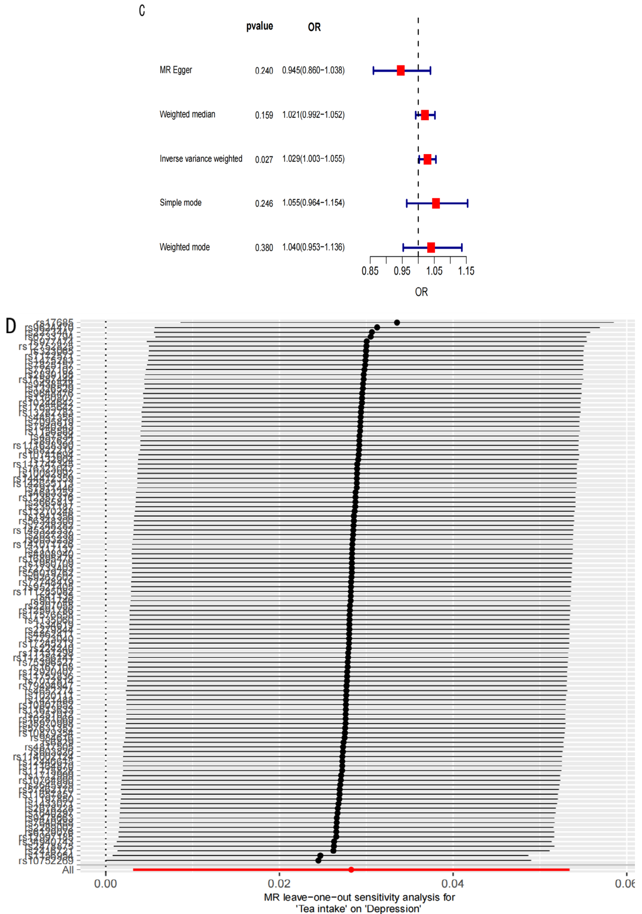
Figure 2. Mendelian randomization analysis (cont.). (A) Funnel plot analysis of the causal association between tea consumption and the risk of depression in a meta-analysis study. (B) MR Scatter plot analysis of causal relationship between tea intake and risk of depression. (C) Forest map of MR Analysis of causal relationship between tea intake and depression risk. (D) Graph of sensitivity analysis result of "leave one method".
