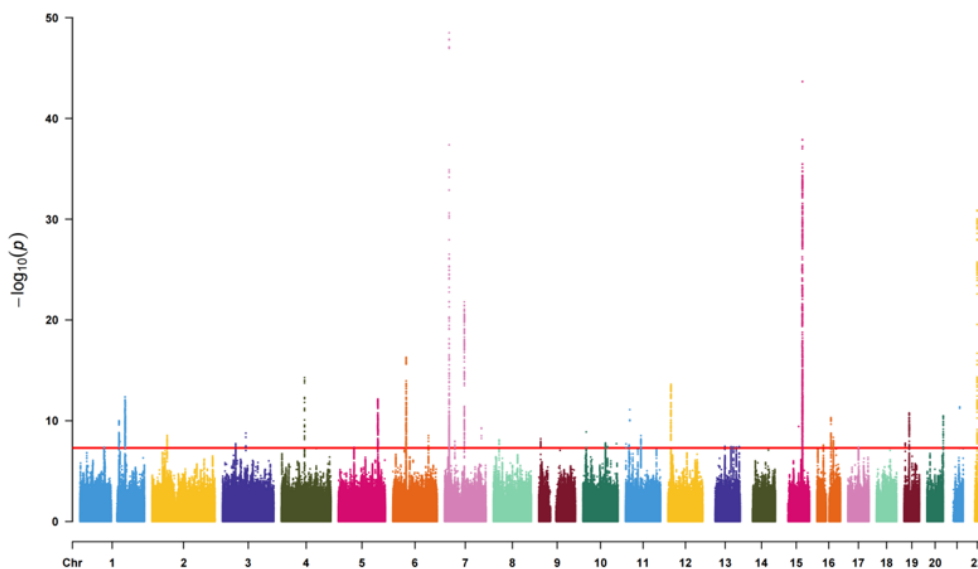
Figure 1. The outcome of IVs selection.
