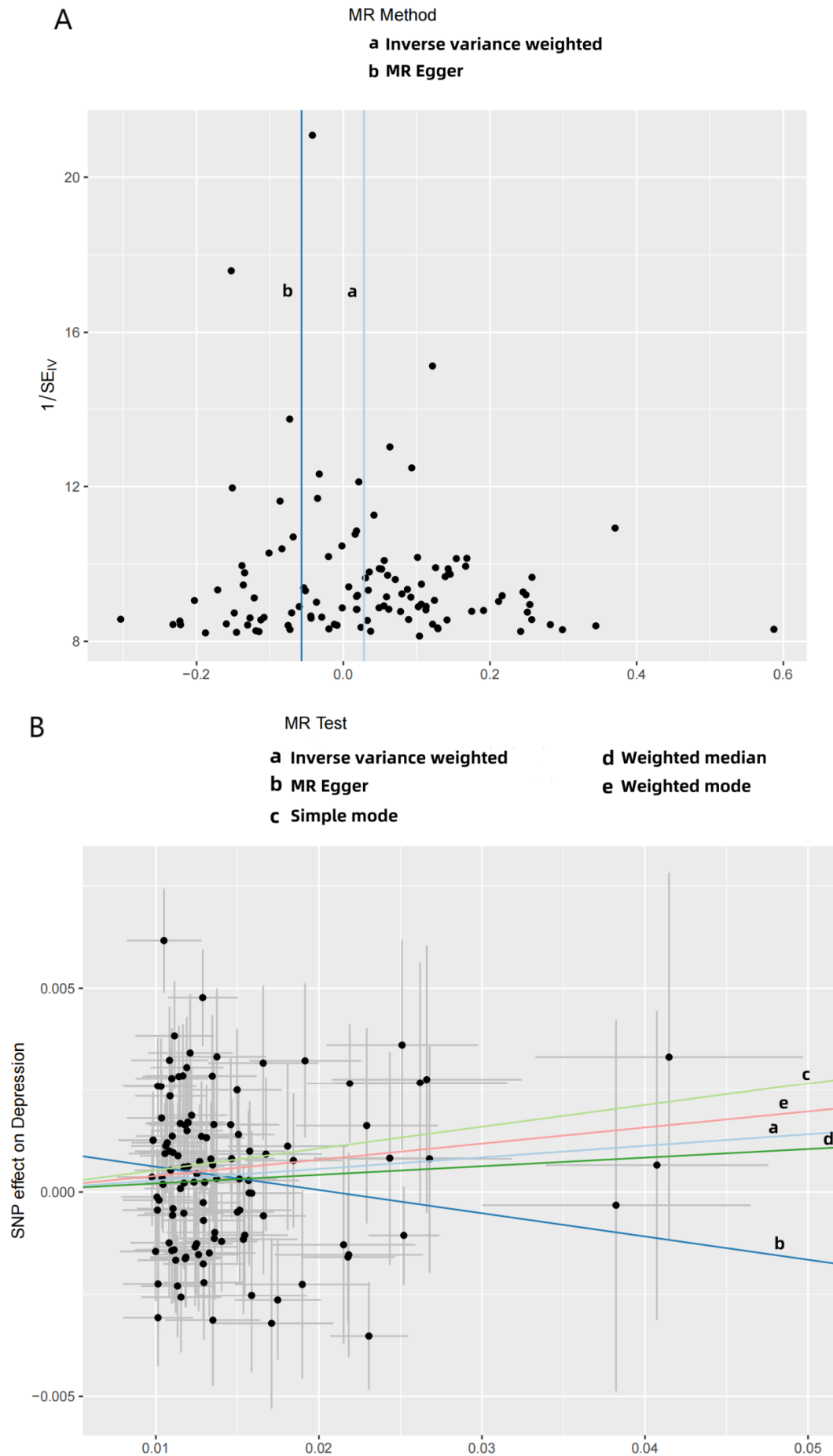
Figure 2. Mendelian randomization analysis. (A) Funnel plot analysis of the causal association between tea consumption and the risk of depression in a meta-analysis study. (B) MR Scatter plot analysis of causal relationship between tea intake and risk of depression. (C) Forest map of MR Analysis of causal relationship between tea intake and depression risk. (D) Graph of sensitivity analysis result of "leave one method".
