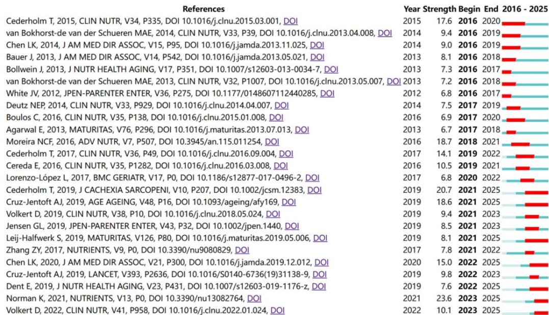
Figure 10. Citation bursts
